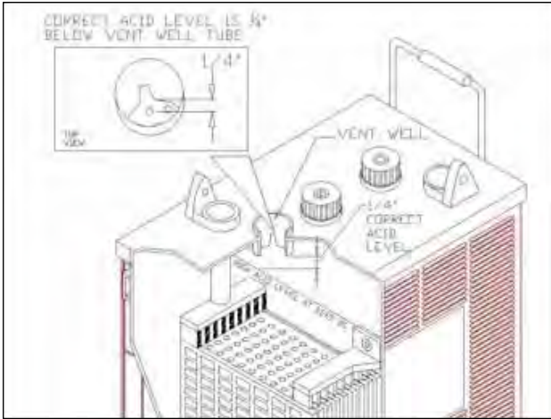
Figure 4 – Electrolyte level
